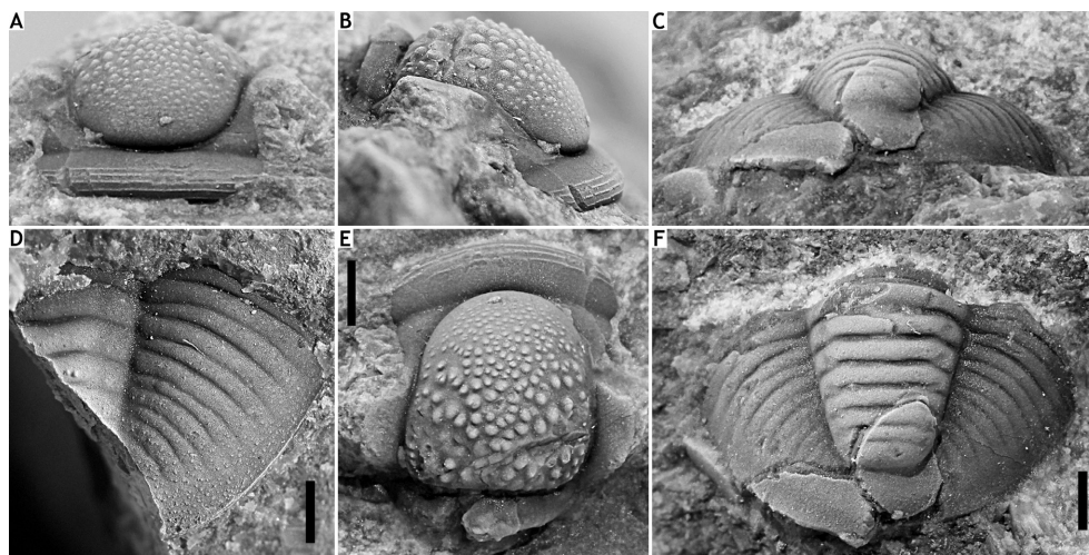
Figure 12. Gerastos silvicultrix sp. nov. from the Heisdorf Formation at B-099, Ahütte.
