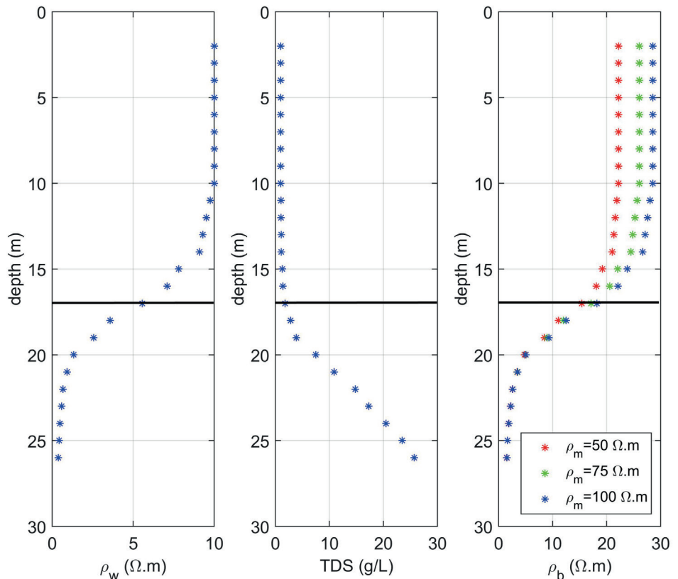
Figure 4. Hypothetical salinity profile and the resulting pore water and bulk resistivity as a function of depth for a range of values of F , \rho_m and f_{11} .
