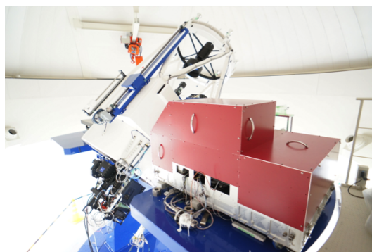
Figure 1: The picture of the NIR high-resolution spectrograph, WINERED (the red box).
