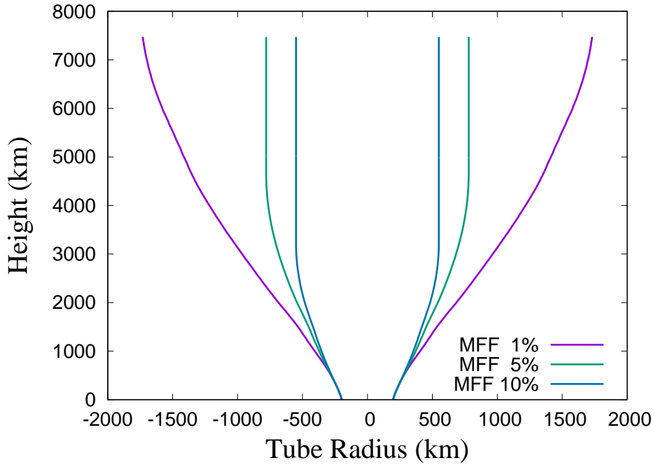
Figure 1: Flux tube models for \beta Hyi based on different magnetic filling factors; see Fawzy and Cuntz (2023) for details. (Reproduced from Fawzy and Cuntz, 2023, originally published by Springer Nature.)
