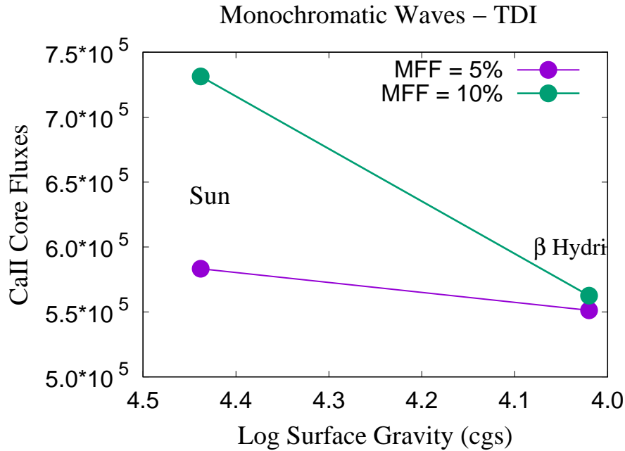
Figure 2: Emergent Ca II core fluxes for two-component chromosphere models (acoustic and magnetic) pertaining to the Sun and \beta Hyi with photospheric magnetic filling factors given as 5% and 10%. (Reproduced from Cuntz and Fawzy (2022) – CC BY 4.0.)
